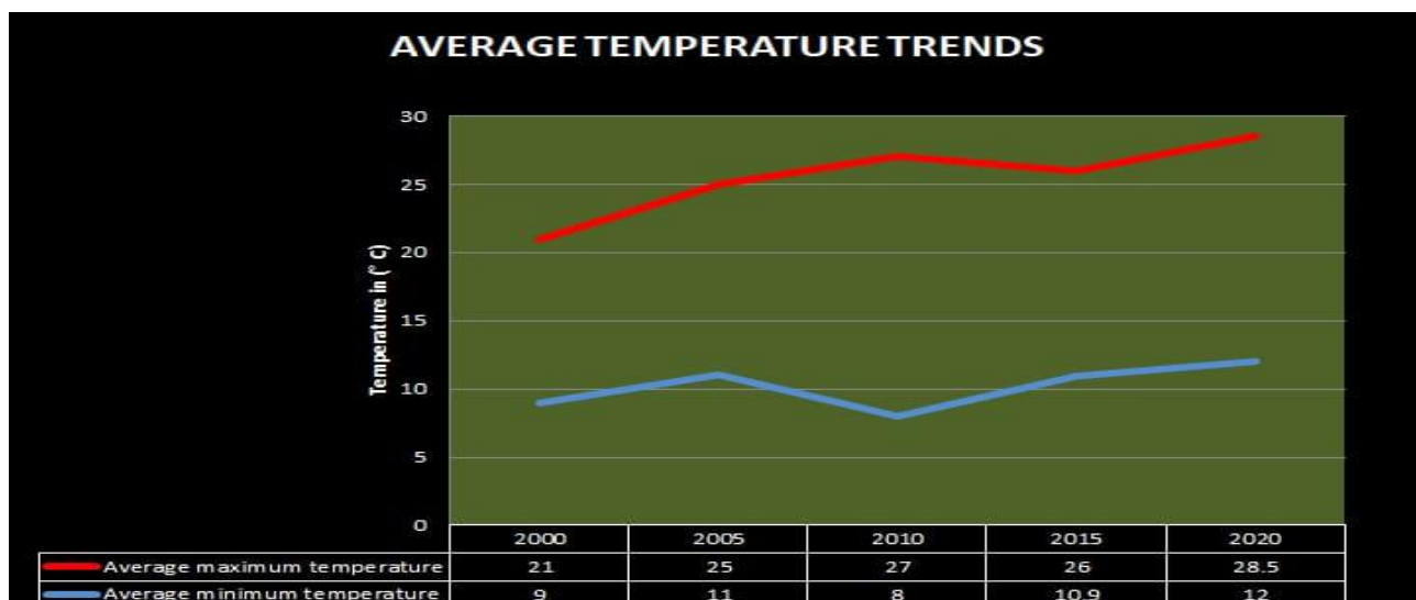
Figure 1: Average temperature trends in the county
